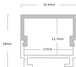
AL-3 with square diffuser
