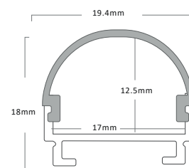
AL-3 with round diffuser
